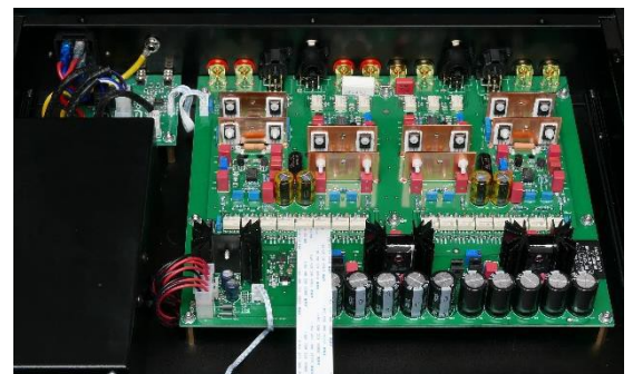
C-102's Mainboard
